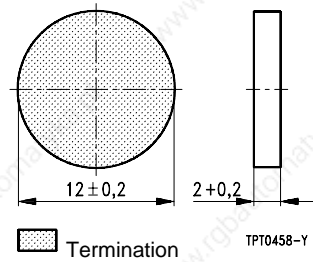
Dimensions (mm)
