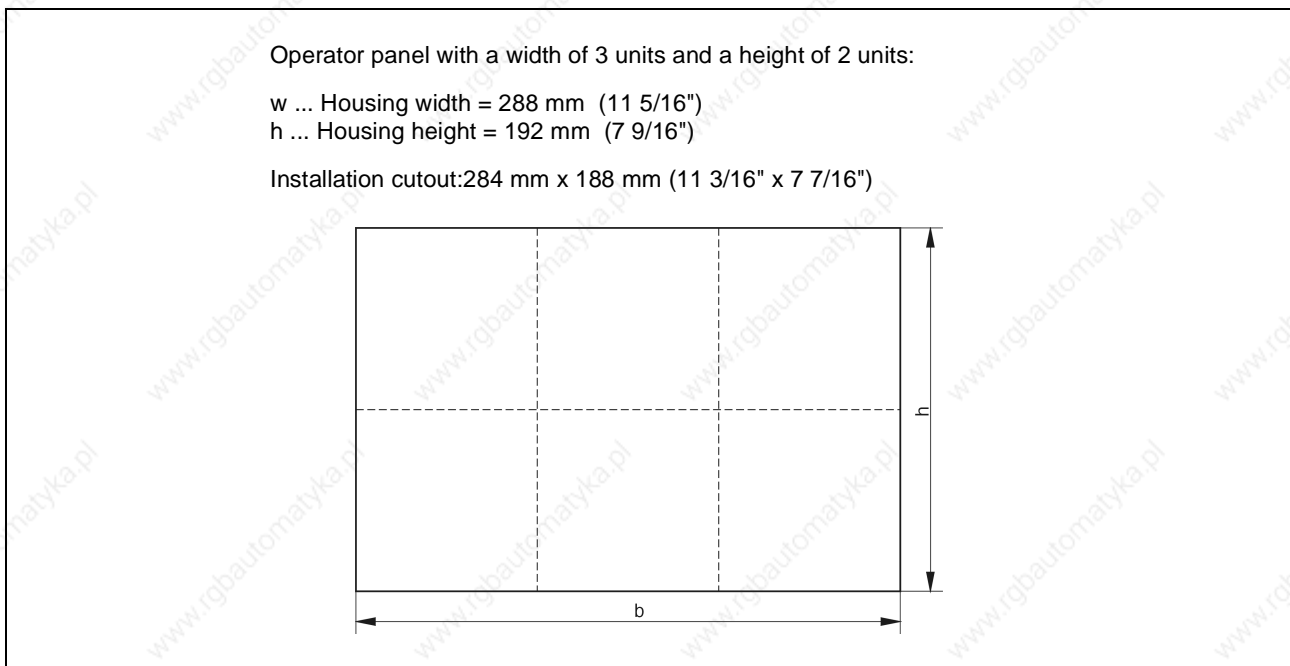
Diagram 5: PANELWARE cutout size example
