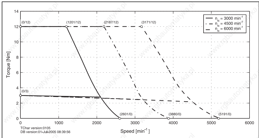
Figure 22: Speed - torque characteristic curve for 8LSA36.eennnffgg-0
