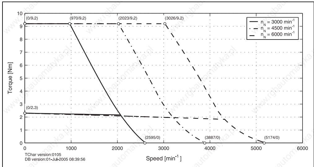
Figure 21: Speed - torque characteristic curve for 8LSA35.eennnffgg-0
