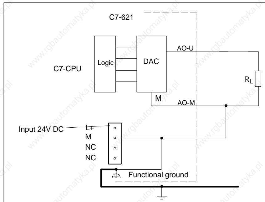
Figure 7-6 Connection of Loads to a Voltage Output of a Non-Floating Analog Output Module
