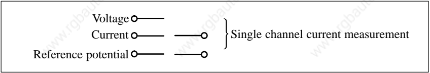
Figure 7-9 Connection of a Channel for Current Measurement
