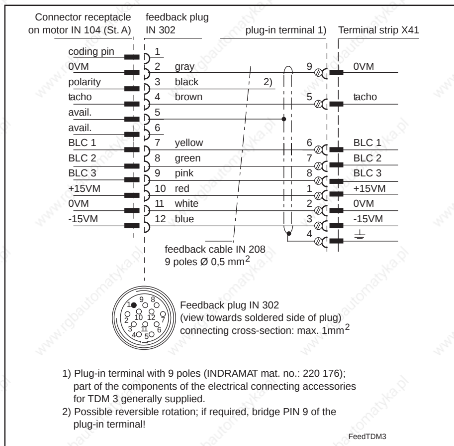
Figure 69: Plug connection of the feedback cables between return unit of the MAC motor and terminal strip of servo drive modules TDM3 and TDM6.
