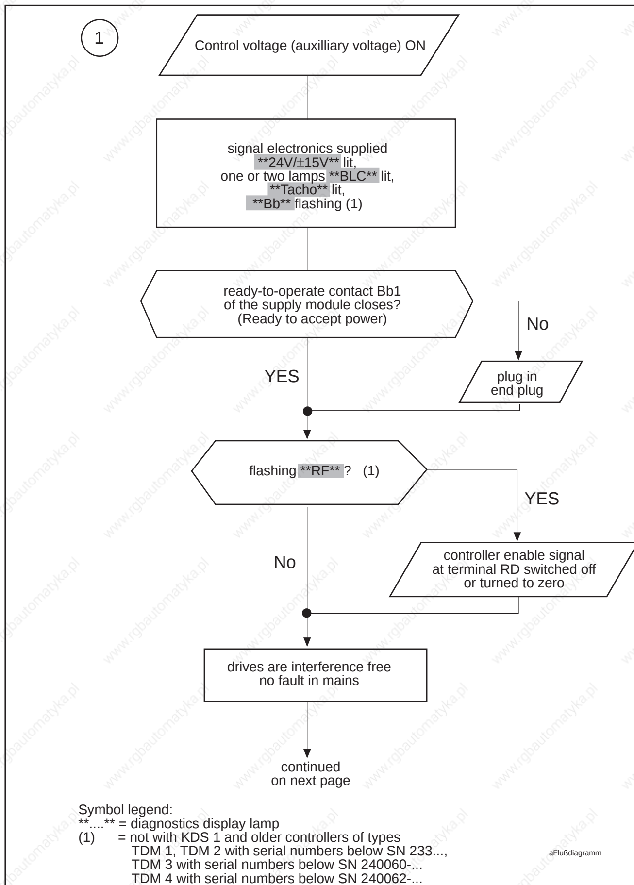
Figure 72: Power-Up Sequence
