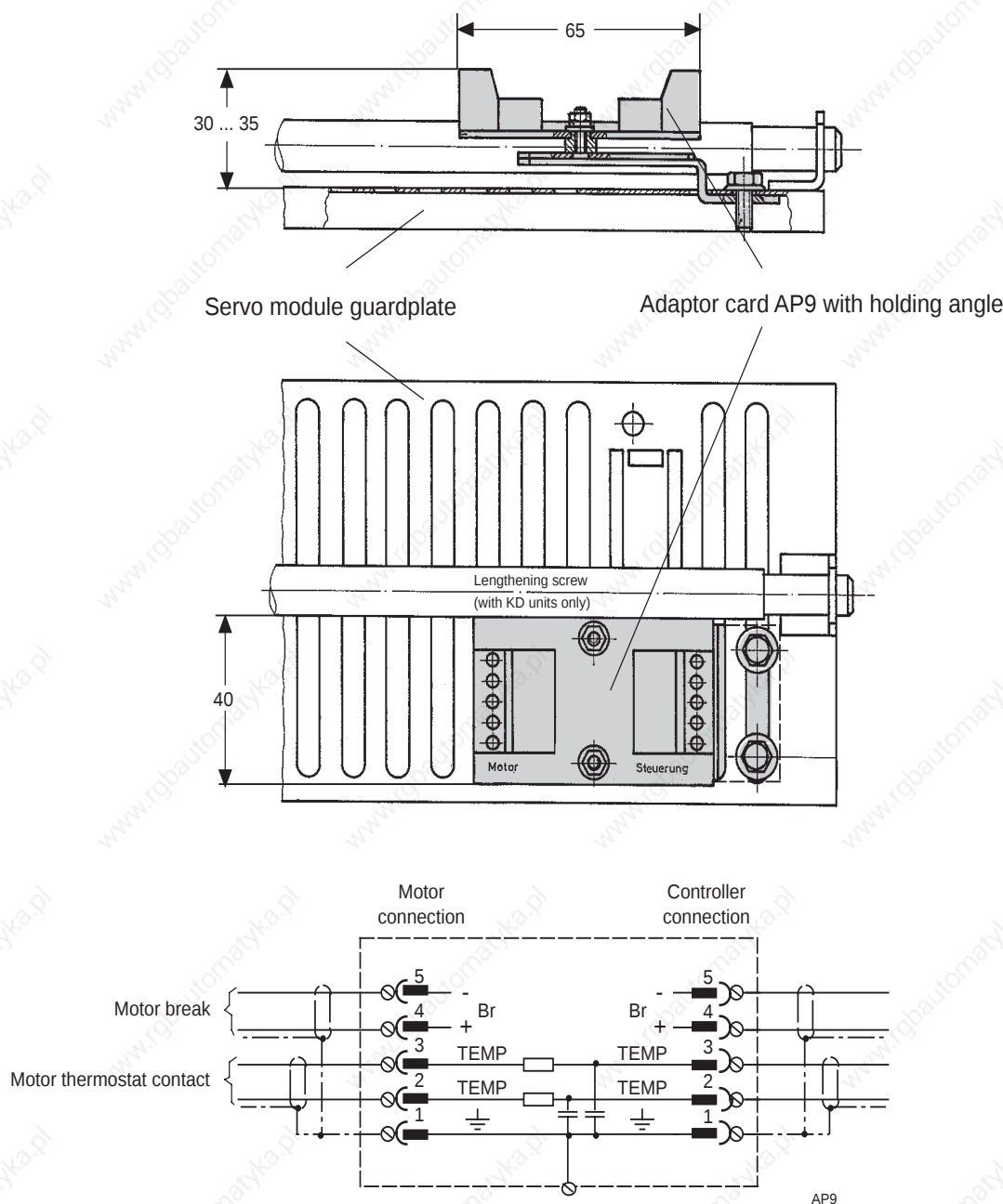
Figure 53: Mounting and connecting adaptor card AP9
