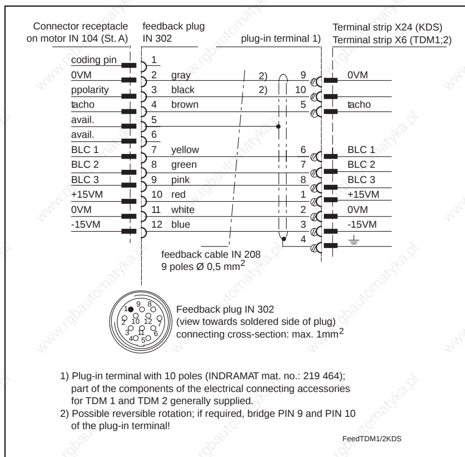
Figure 68: Plug connection of the feedback cable between the return unit of the MAC motor and the terminal strip of servo drive modules TDM1, TDM2 or KDS1.
