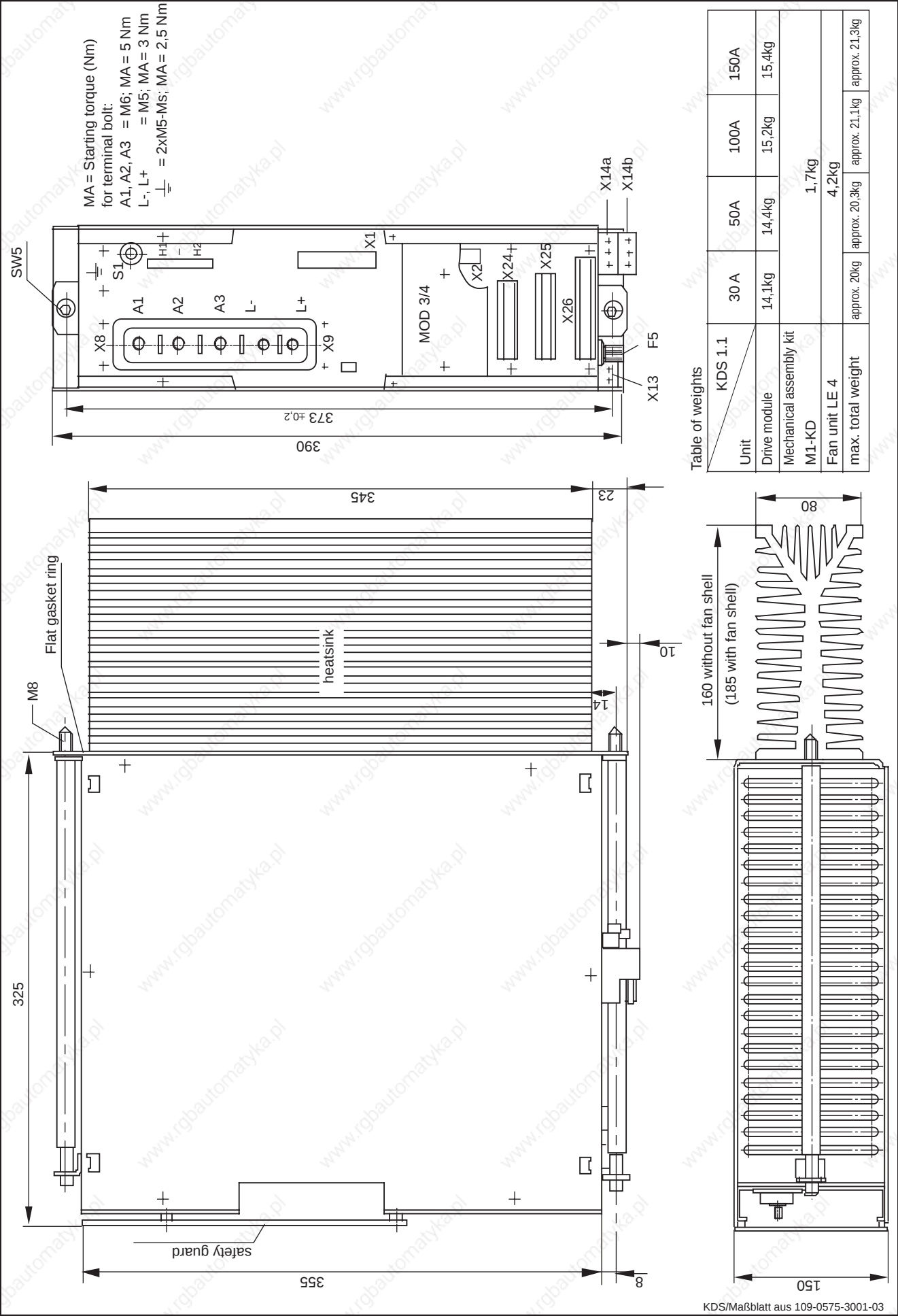
Figure 49: Dimension sheet for KDS1
