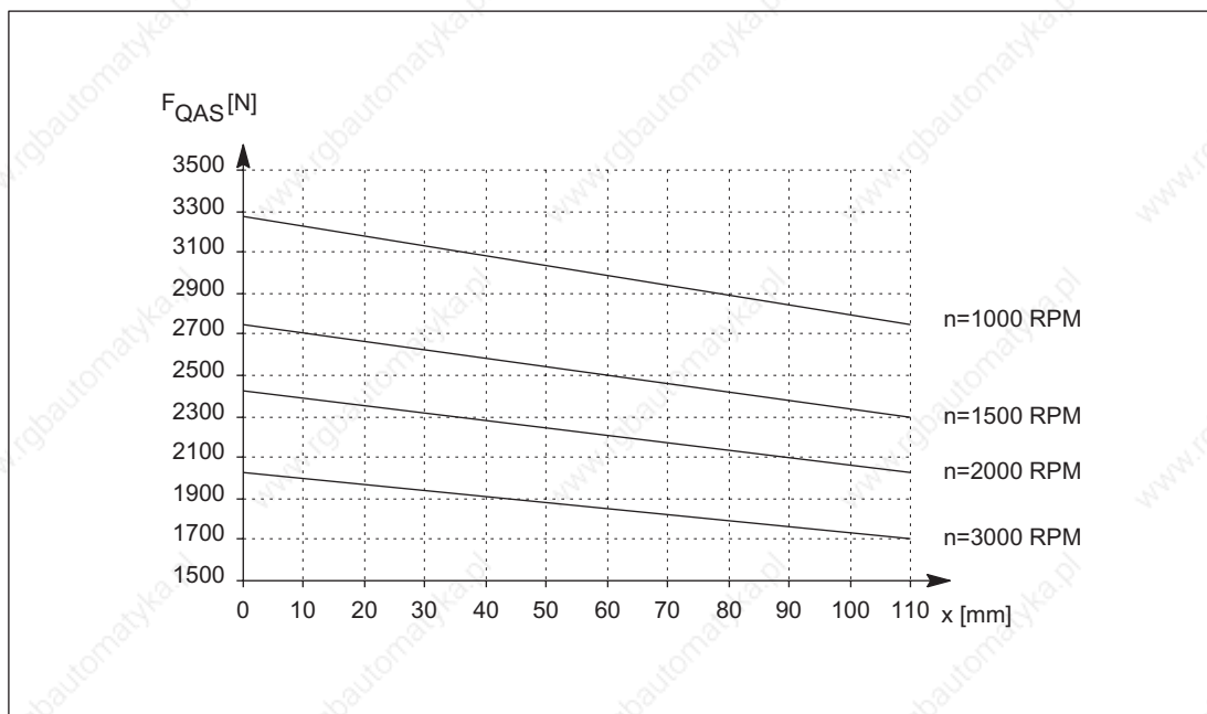
Figure 3-114 Cantilever force F_Q at a distance x from the shaft shoulder for a nominal bearing lifetime of 20,000 h
