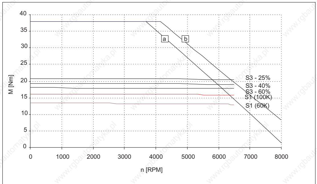
Figure 3-83 Speed-torque diagram 1FT6064-6WK7□
