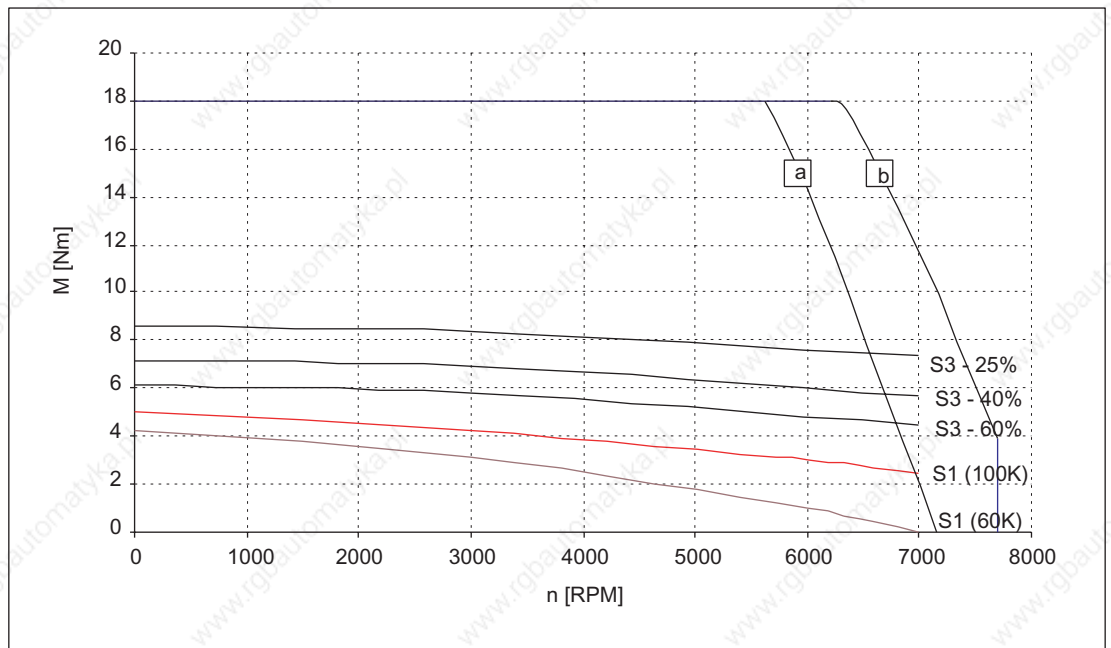
Figure 3-8 Speed-torque diagram 1FT6044-4AK71
