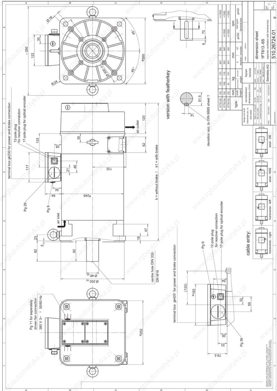
Figure 5-31 1FT613 force-ventilated with terminal box
