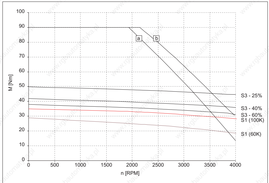
Figure 3-56 Speed-torque diagram 1FT6086-8SF7□
