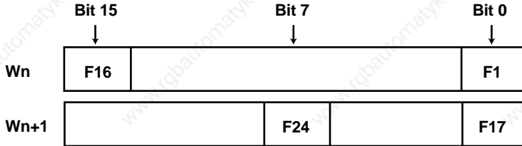
Figure 35: Wn and Wn+1, Word Structure
