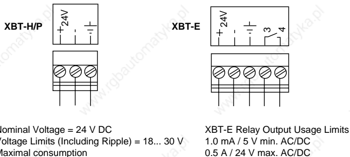
Figure 30: Power Supply and Relay Connections
