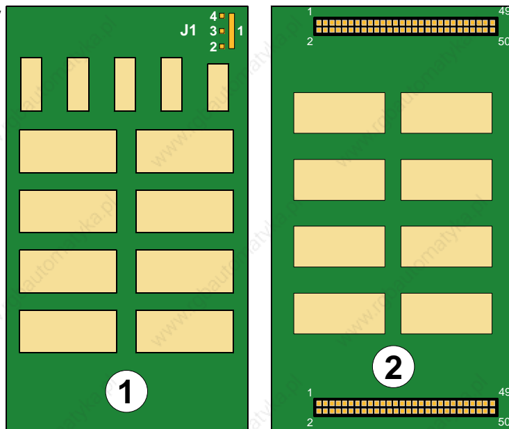
Figure A-1: DM600 Memory Piggyback
