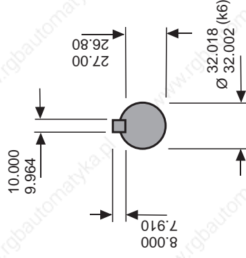
SHAFT END DETAIL
