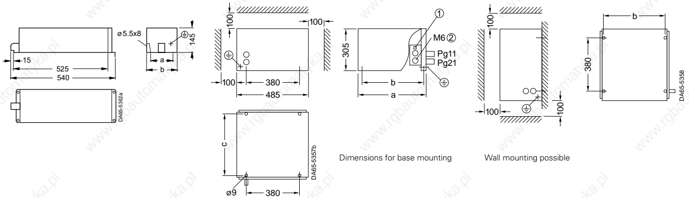
Braking resistor 5 kW and 10 kW
