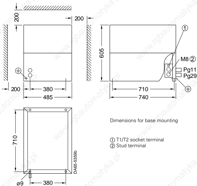
Braking resistor 100 kW 6SE7031-6ES87-2DC0
