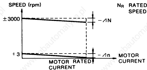
Fig 10 2 Speed Regulation
