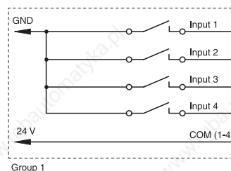
Source Circuit:
