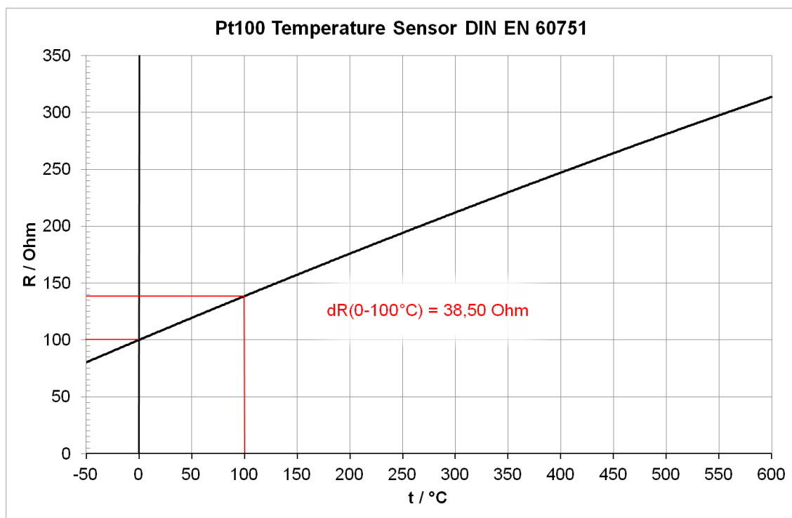
Figure 1: Resistance characteristics
