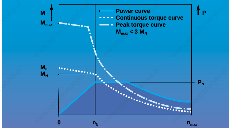
Motor performance curve
