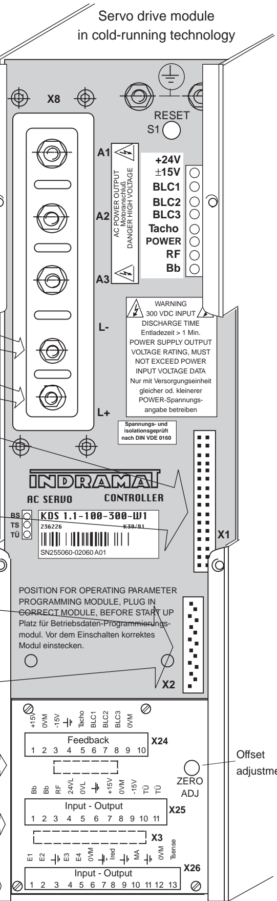
Figure 40: Front view of servo drive module KDS1 with accessories
