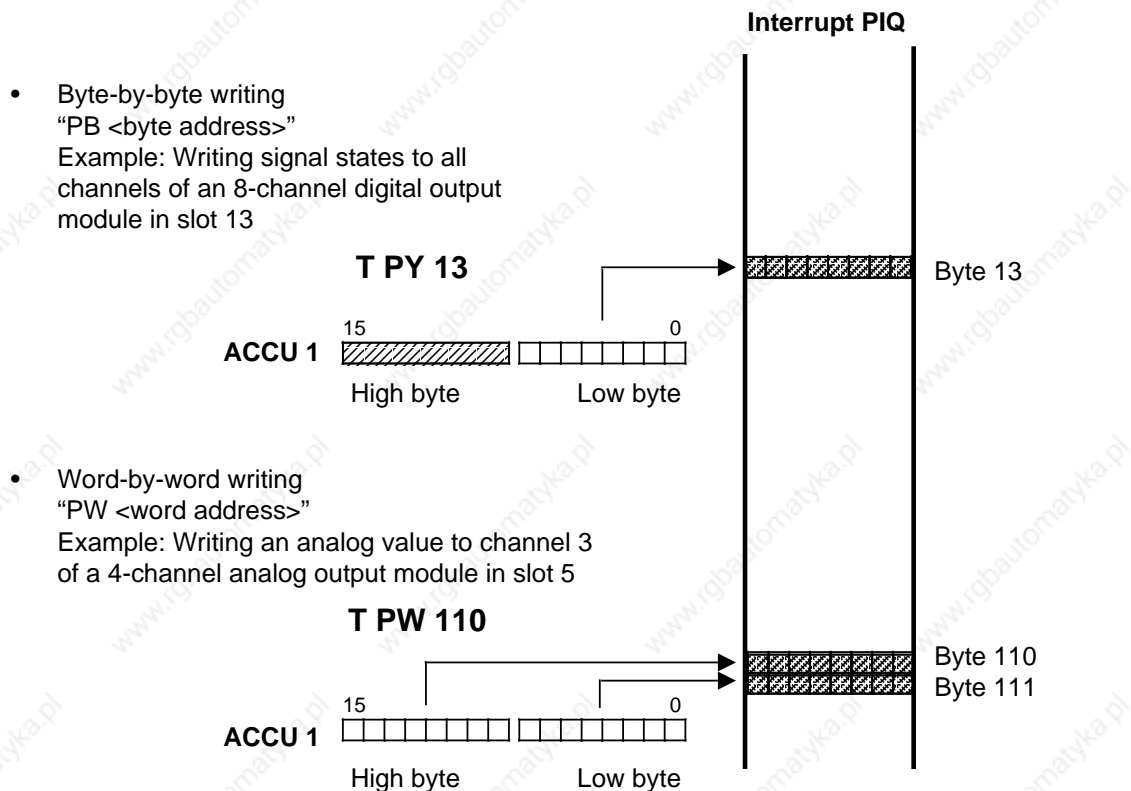
Figure 6-11. Accesses to the Interrupt PIQ
