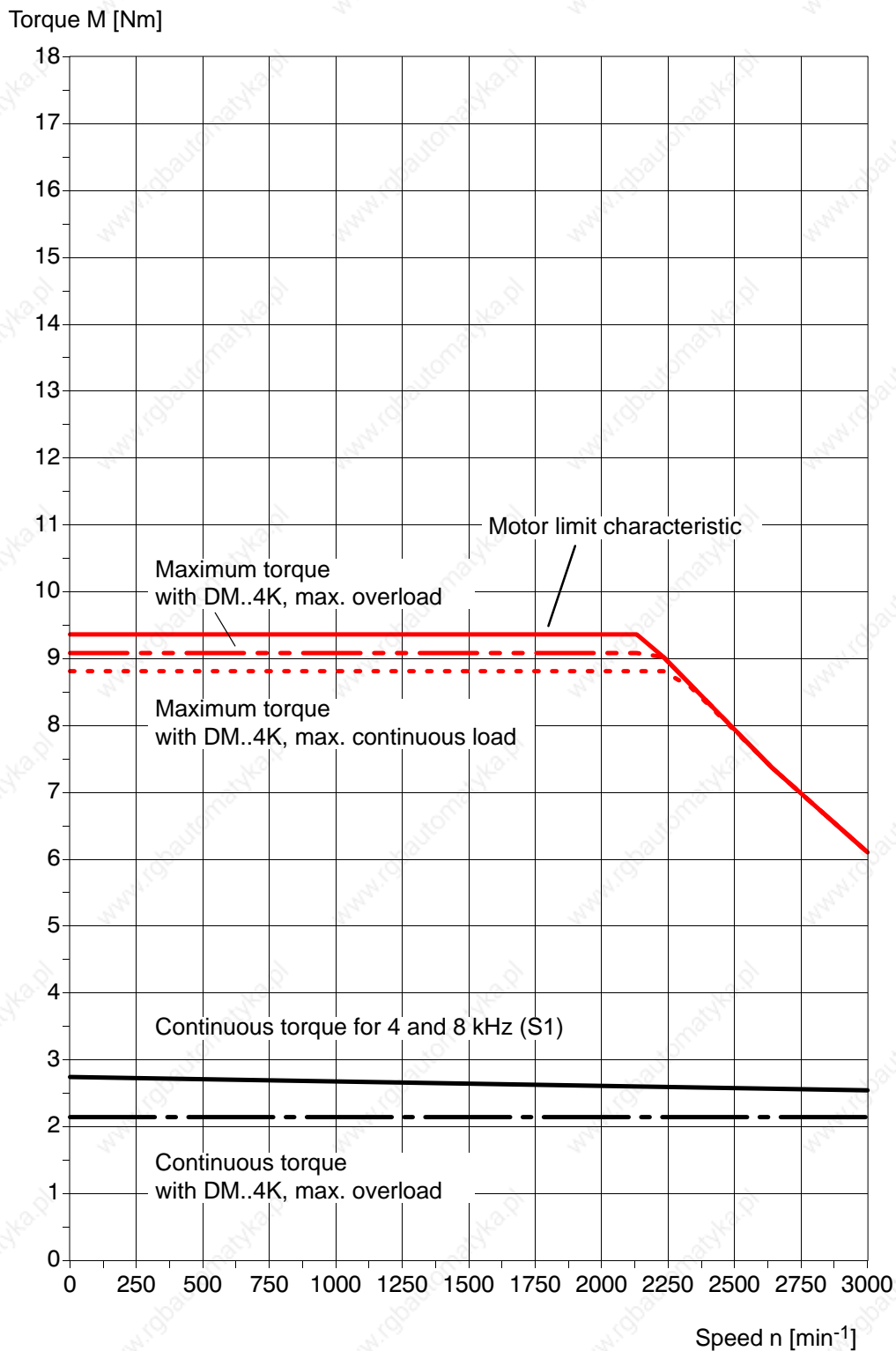
Continuous torque with DM..4K, max. continuous load \triangleq S1 characteristic.
