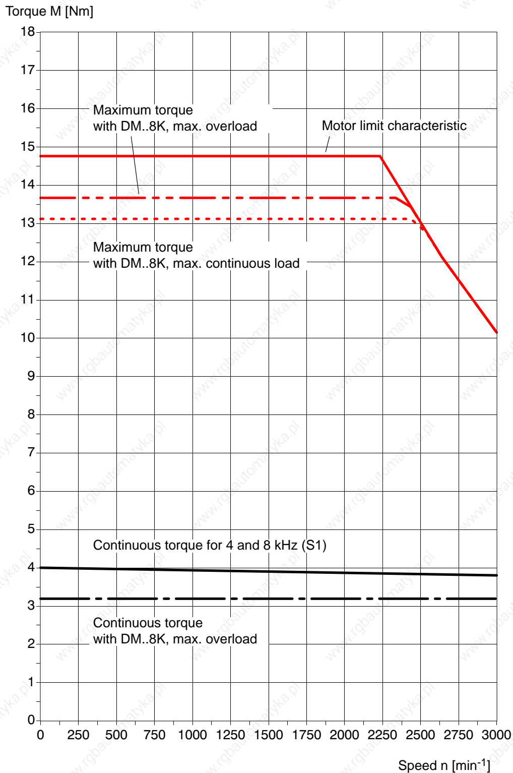
Continuous torque with DM..8K, max. continuous load \triangleq S1 characteristic.
