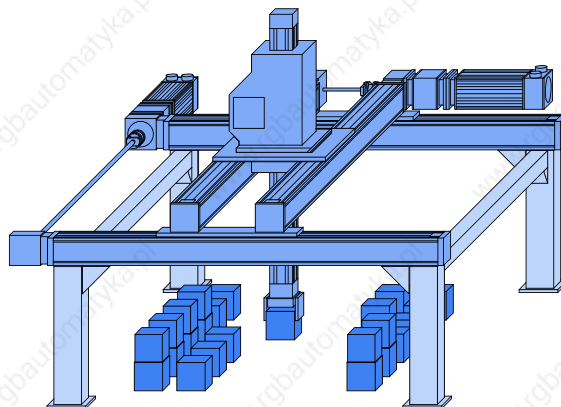
Gantry robots
