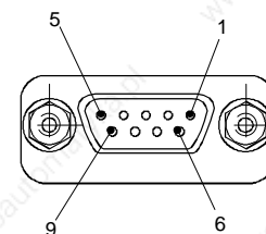
9 pin SUB-D plug connector (DIN 41652)
