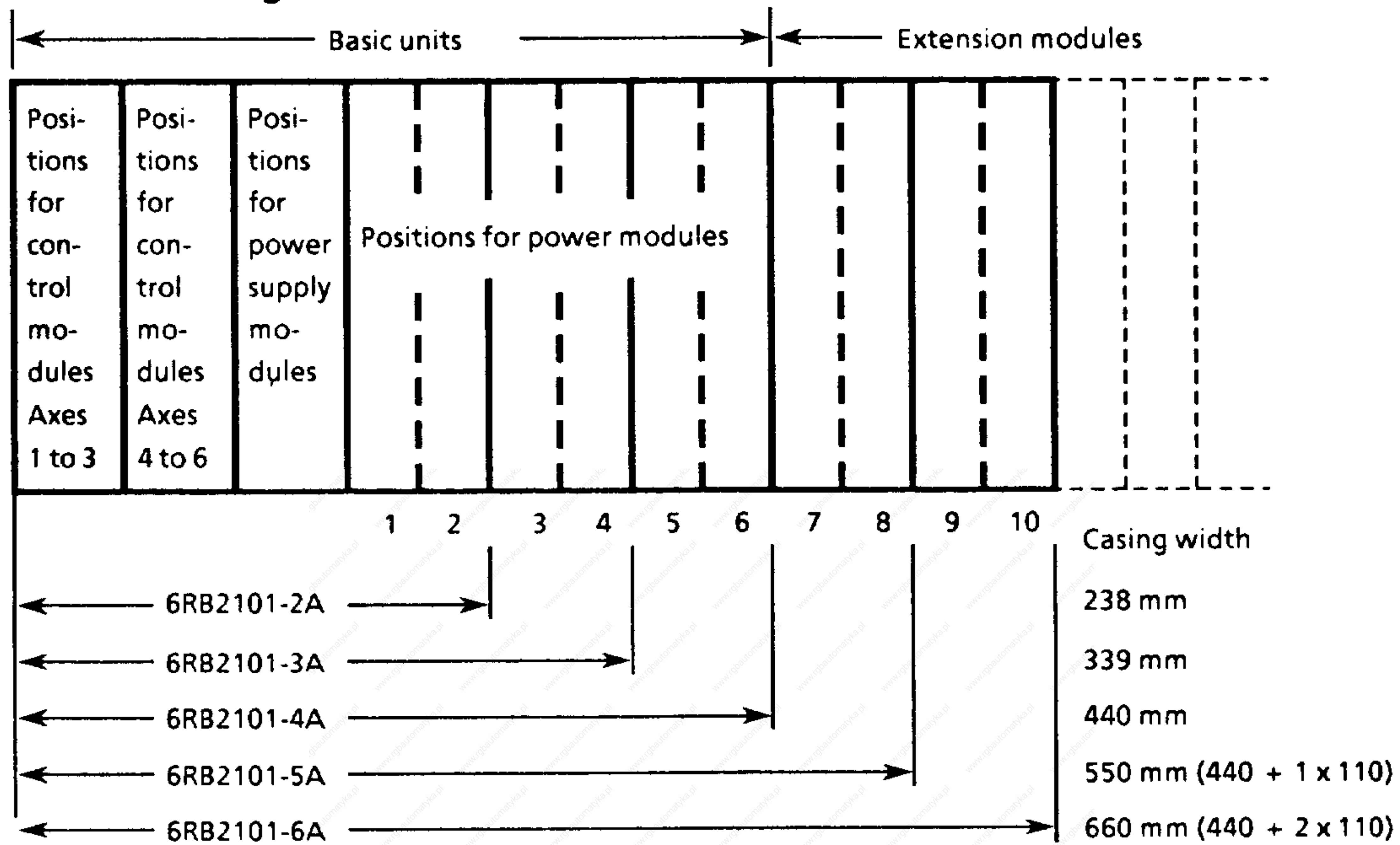
Fig. 1.2 Casing
