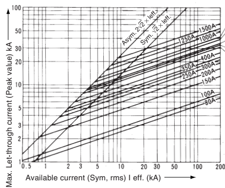
Current-limiting characteristic
