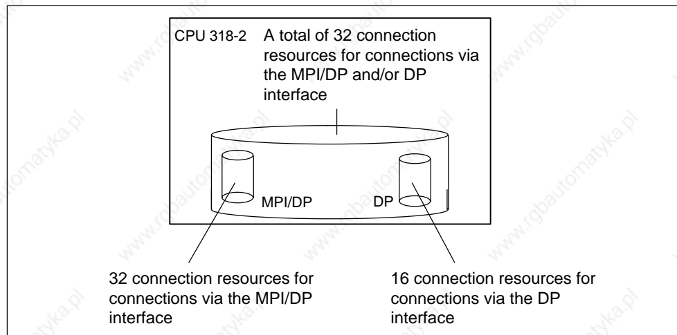
Figure 1-3 Principle of Connection Resource Allocation for CPU 318-2
