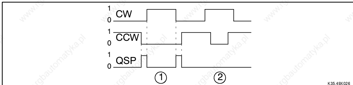
FIG 5-6 Selection of direction of rotation
