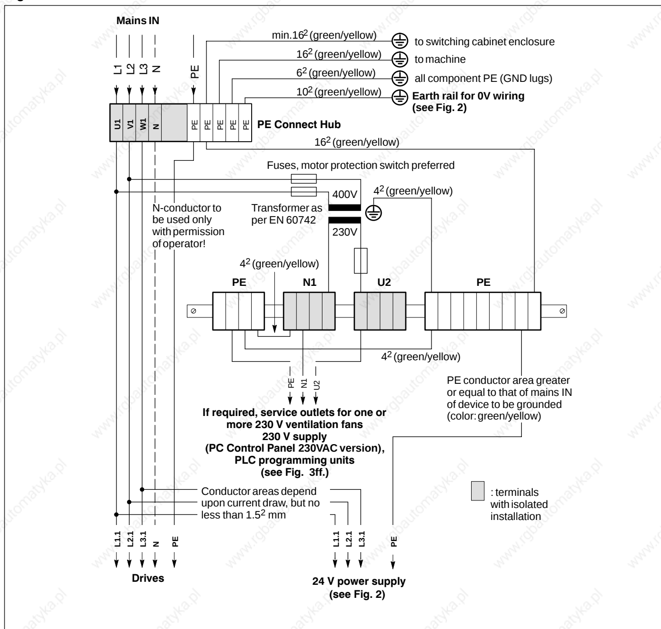
Fig. 1: Mains Connection
