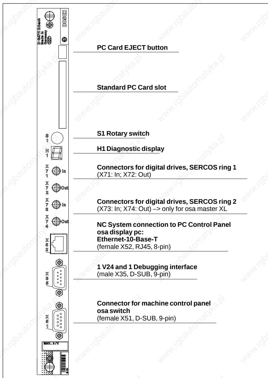
Front view of osa master XL
