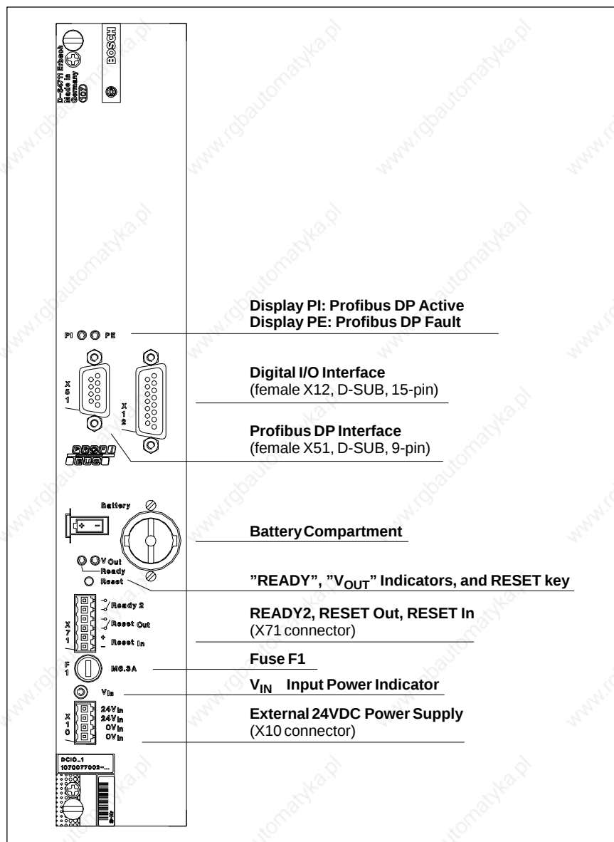
osa dc interface (front view)
