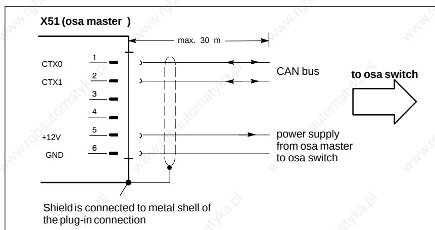
X51 pin assignment (osa master)
