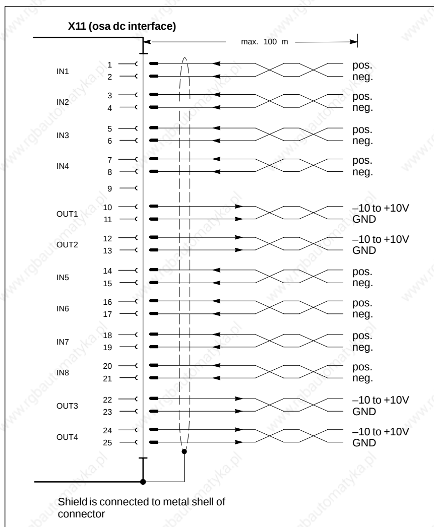
Connector X11 (osa dc interface)
