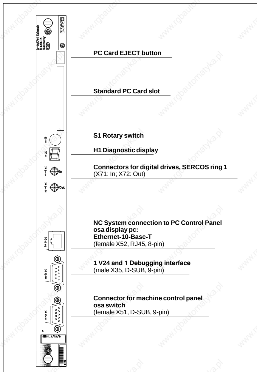
Front view of osa master L
