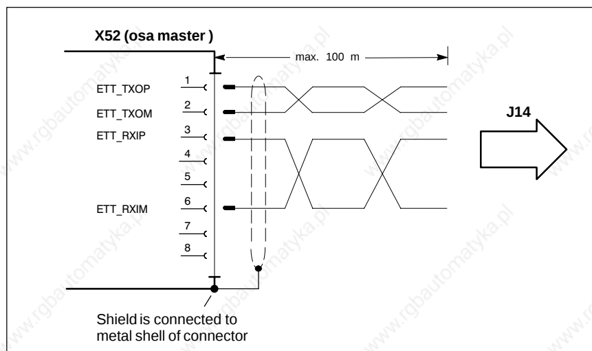
X52 pin assignment (osa master)
