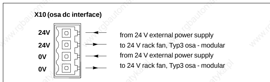
Connector X10 (osa dc interface)
