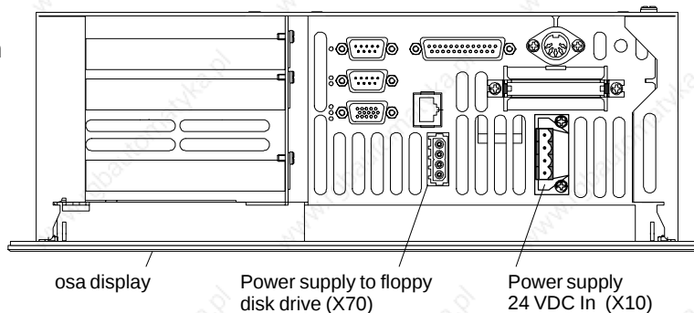
Interface: Power supply 24 VDC In
