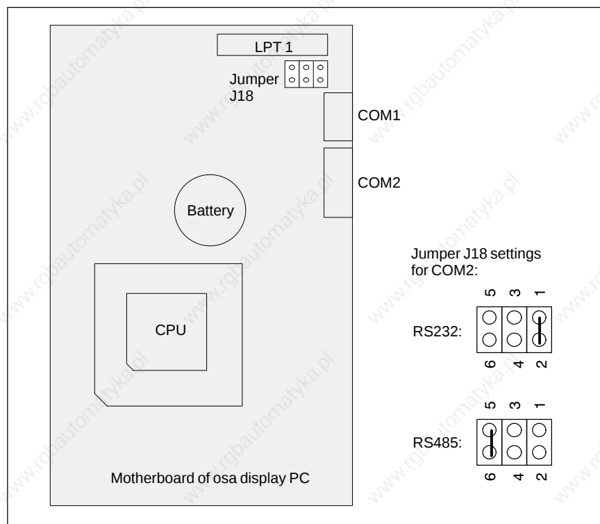
Motherboard jumper settings for COM2
