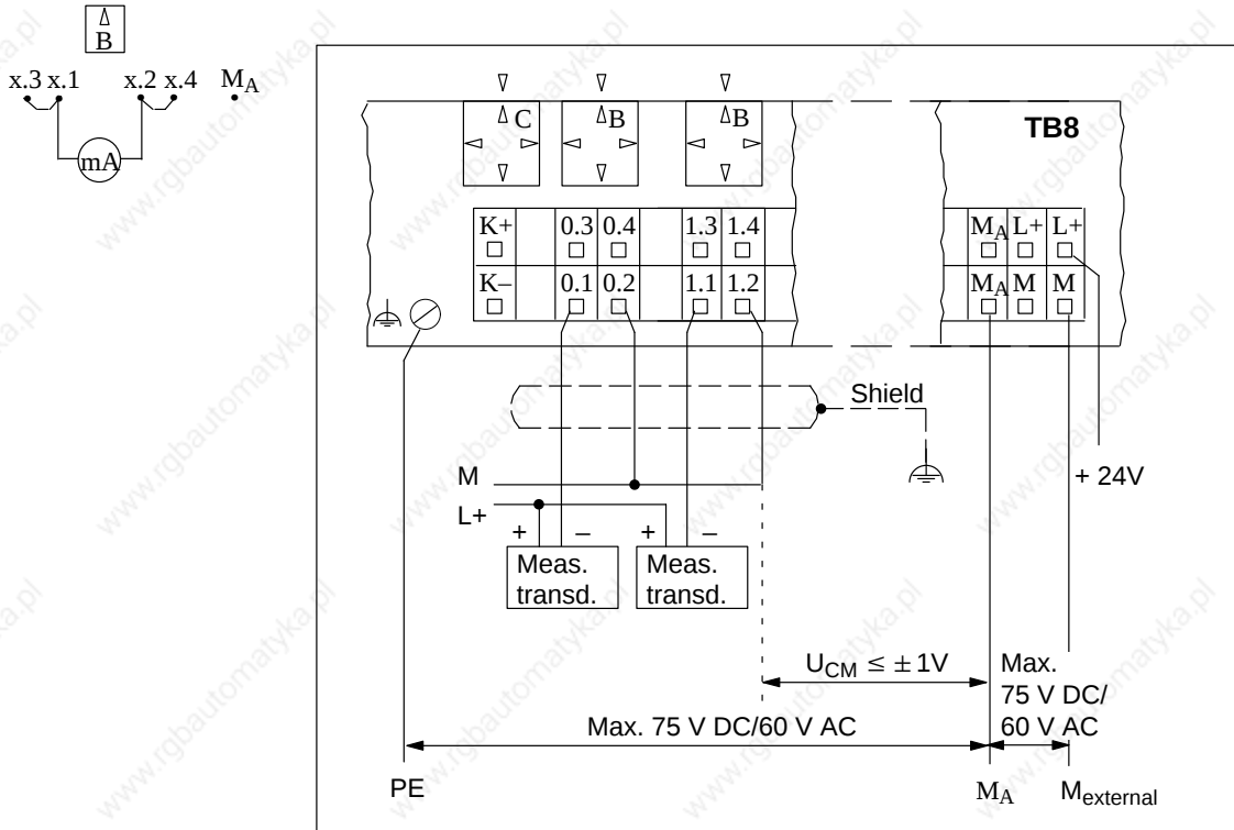
Figure 8-21 Connection of 2-Wire Measuring Transducer as Current Sensor
