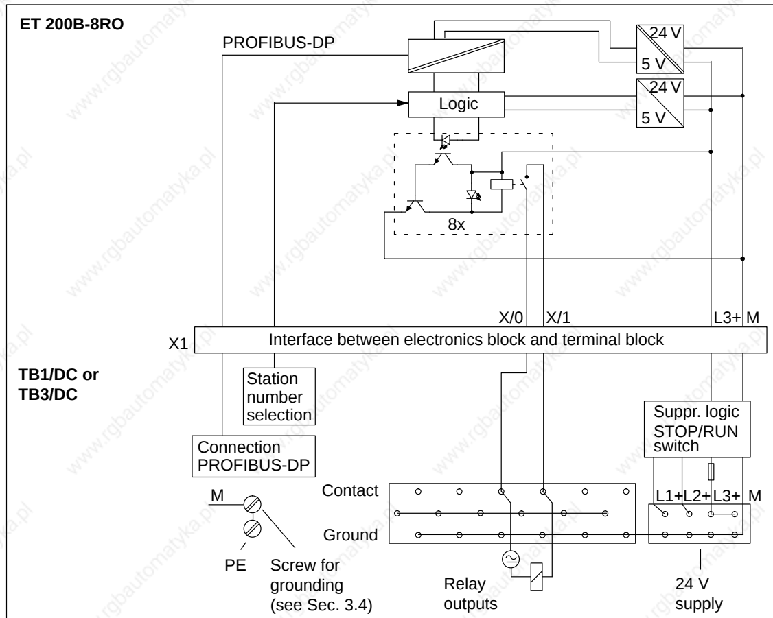
Figure 7-36 Block Diagram: ET 200B-8RO (6ES7 132-0GF00-0XB0) and TB1/DC or TB3/DC
