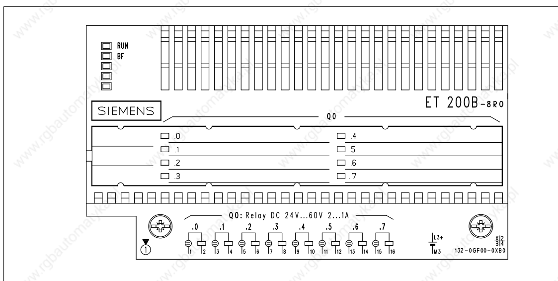
Figure 7-35 Front Elevation: ET 200B-8RO (6ES7 132-0GF00-0XB0)
