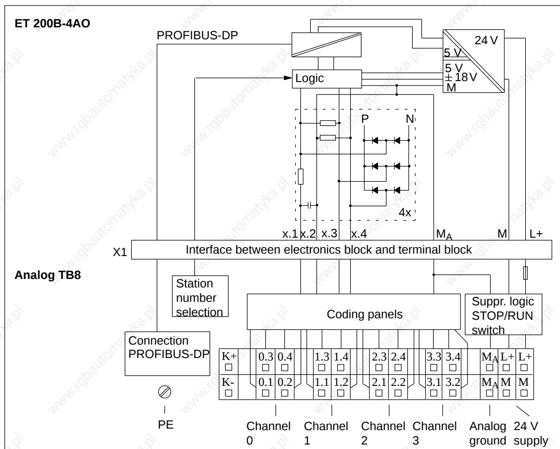
Figure 8-28 Block Diagram: ET 200B-4AO (6ES7 135-0HF01-0XB0) and TB8
