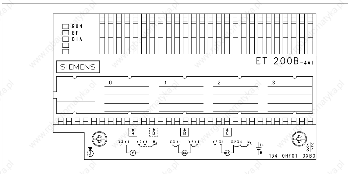
Figure 8-16 Front Elevation: ET 200B-4AI (6ES7 134-0HF01-0XB0)
