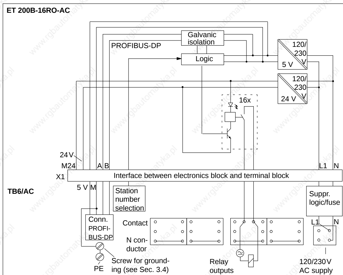
Figure 7-55 Block Diagram: ET 200B-16RO-AC (6ES7 132-0HH00-0XB0) and TB6/AC
