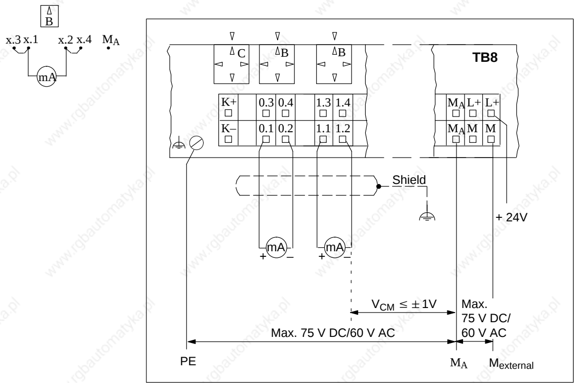
Figure 8-19 Two-Wire Connection of Current Sensors (Floating-Ground Measurement)
