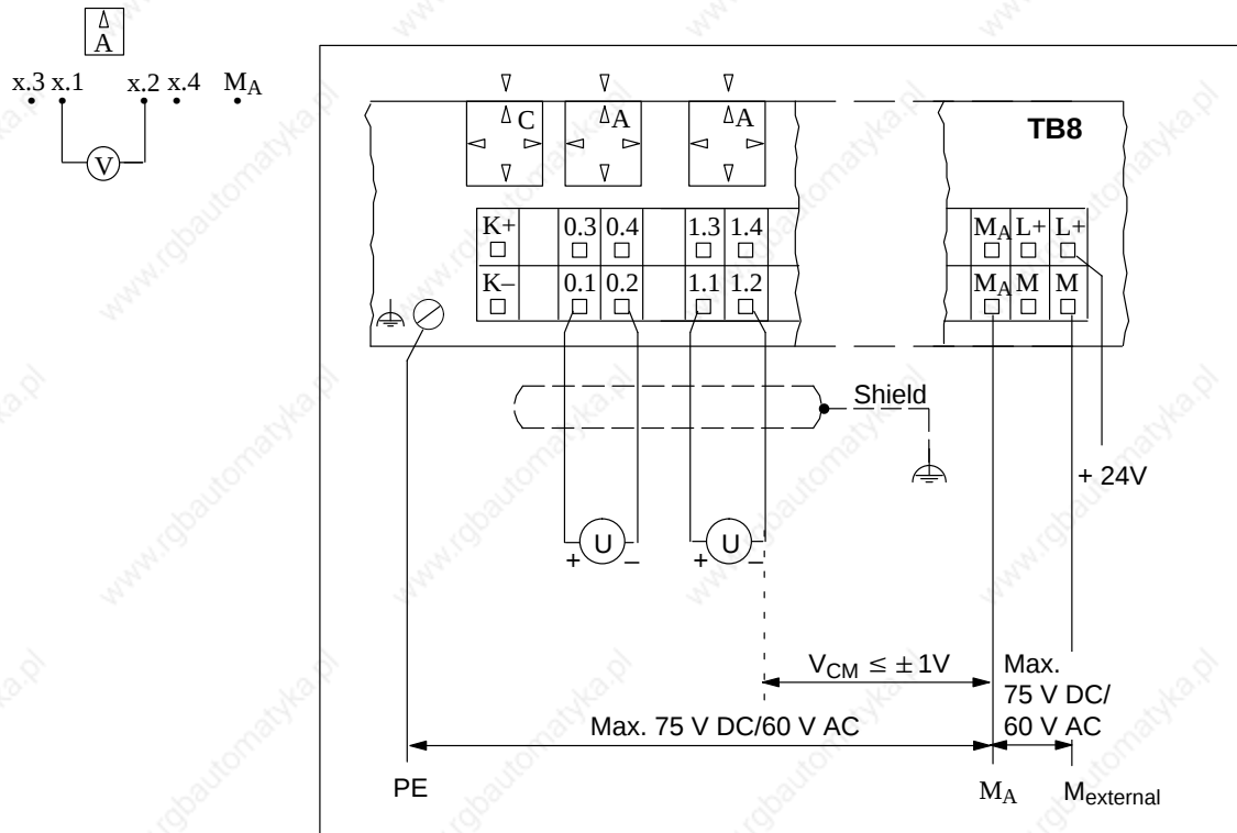
Figure 8-17 Two-Wire Connection of Voltage Sensors to ET 200B-4AI (Floating-Ground Measurement)
