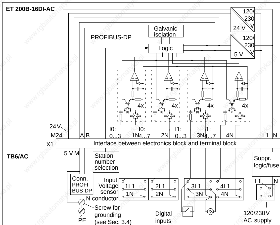
Figure 7-51 Block Diagram: ET 200B-16DI-AC (6ES7 131-0HF00-0XB0) and TB6/AC
