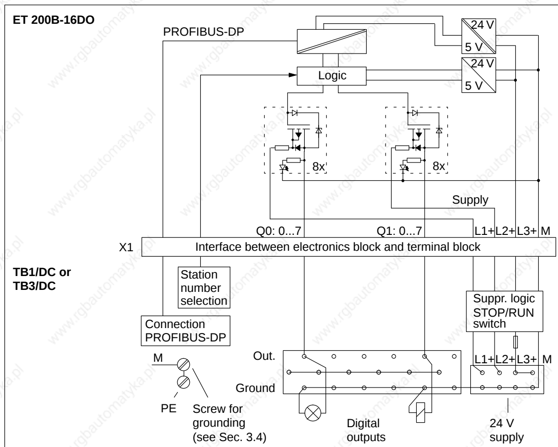
Figure 7-27 Block Diagram: ET 200B-16DO (6ES7 132-0BH01-0XB0) and TB1/DC or TB3/DC
