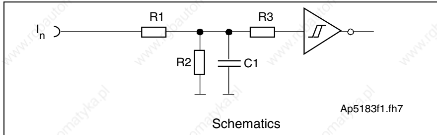
R1: 10k R2: 3k3 R3: 10k C1: no data Fig. 5-39: Input circuit
