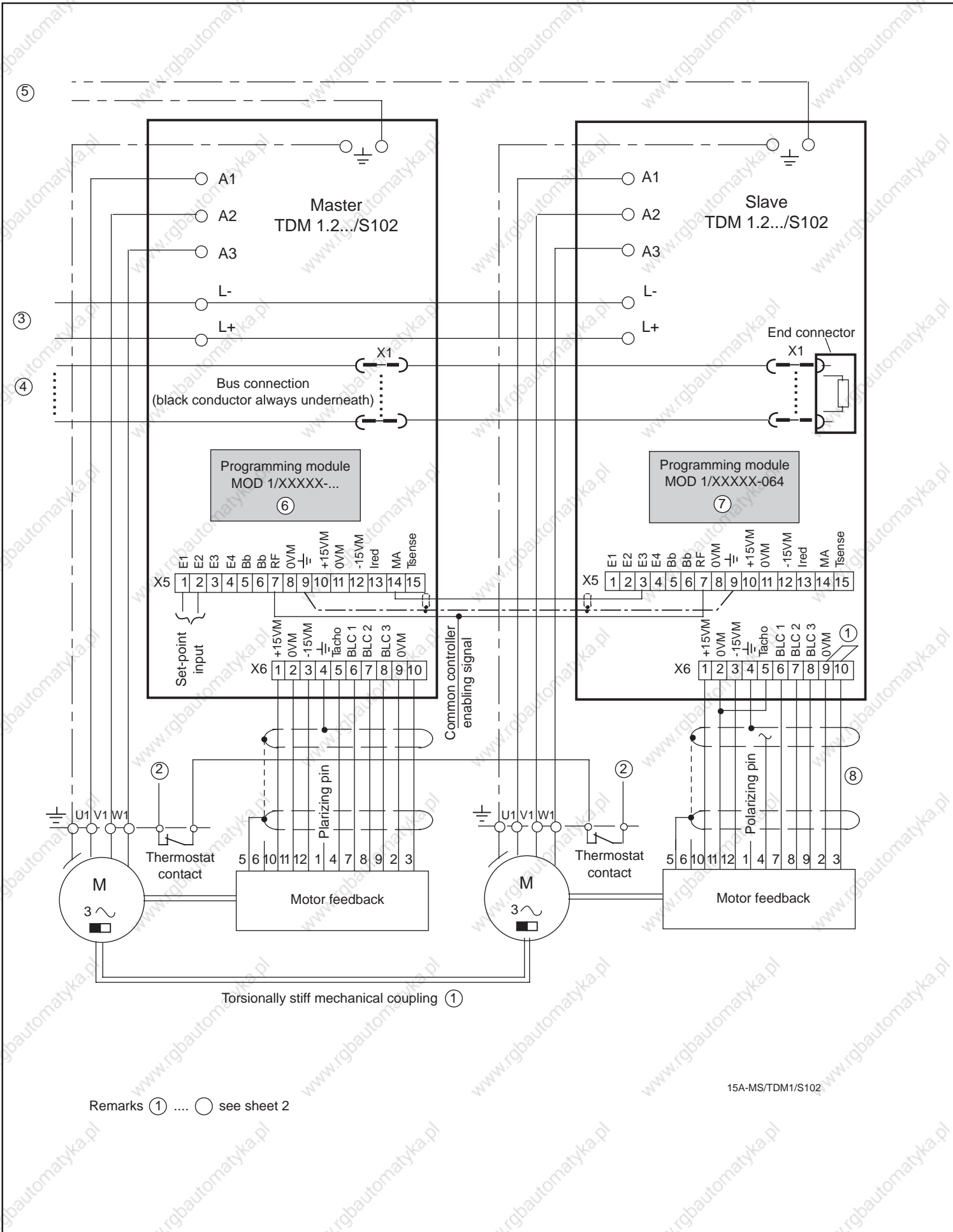
Fig. 15: Master-slave drive with TDM 1.2.../S102
