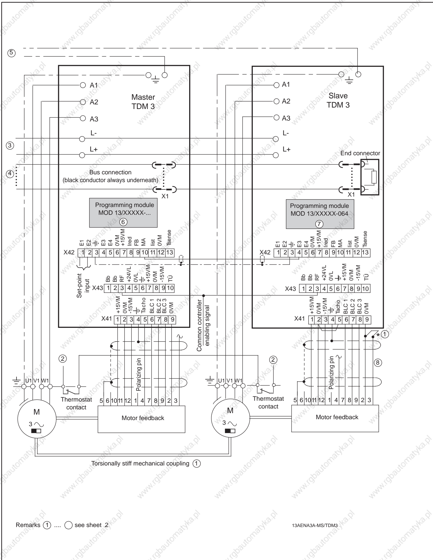
Fig. 13: Master-slave drive with TDM 3
