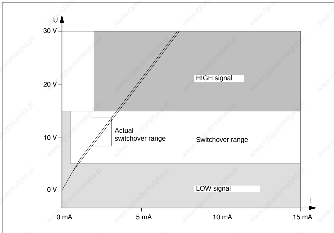
U/I - Characteristic curve
