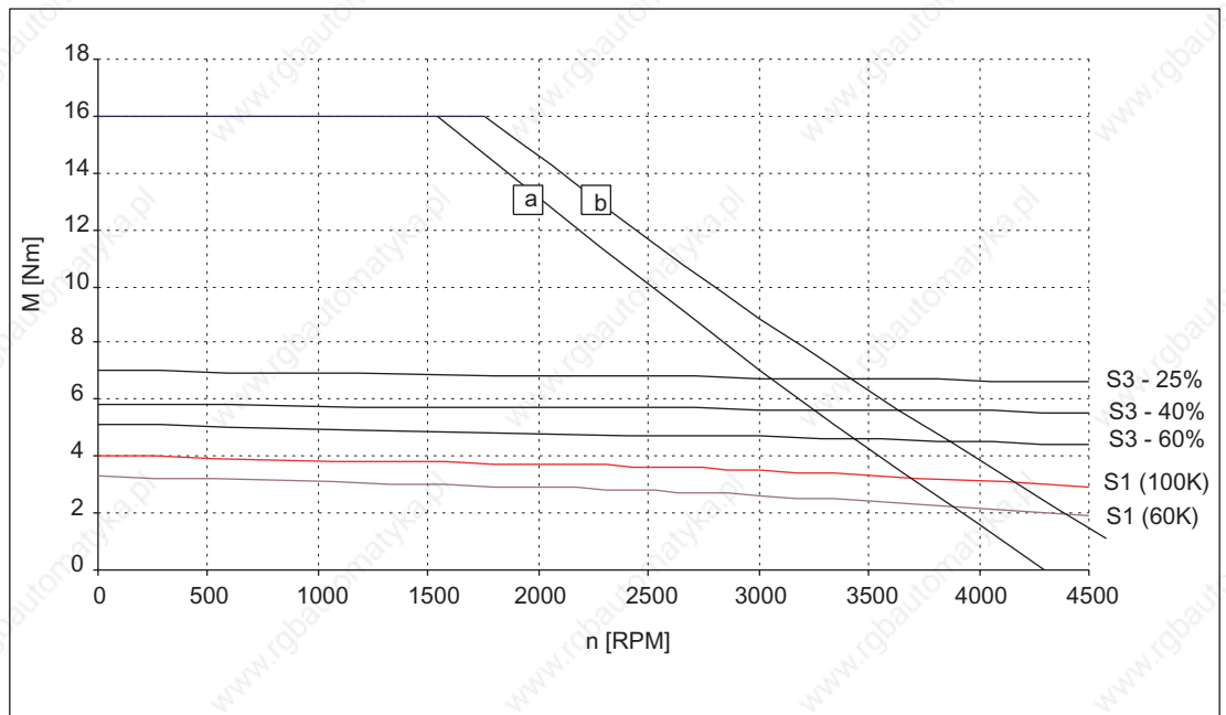
Figure 3-10 Speed-torque diagram 1FT6061-6AF7□
