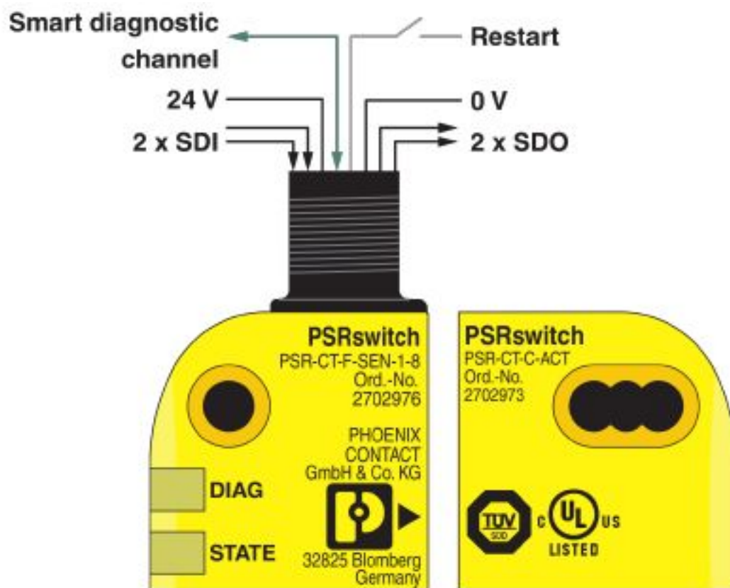
Application drawing
