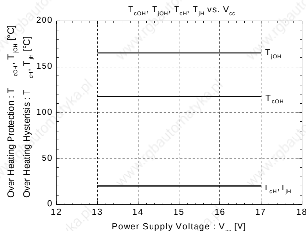
Over Heating Characteristics
