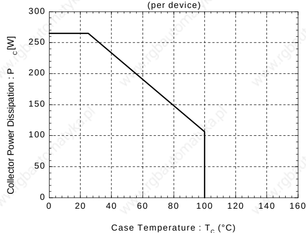
Power Derating For FWD (per device)
