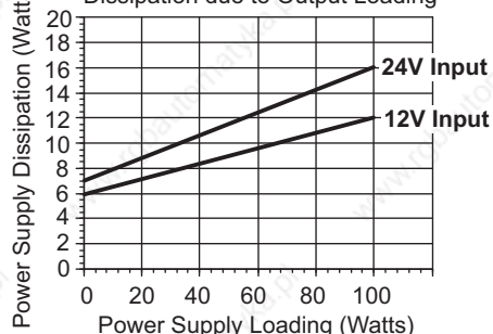
1746-P7 Power Supply Change in Power Dissipation due to Output Loading
