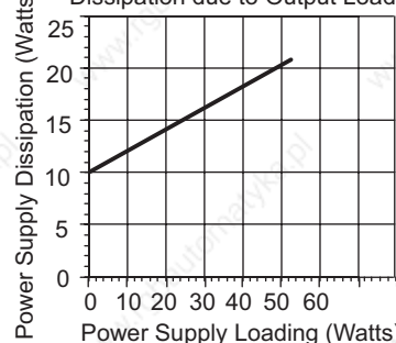
1746-P6 Power Supply Change in Power Dissipation due to Output Loading
