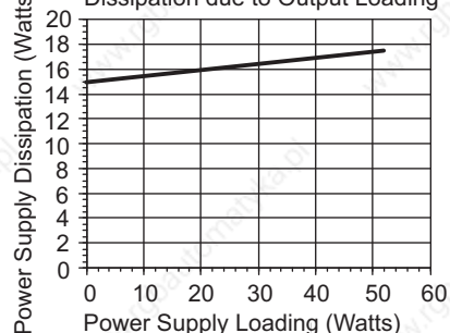
1746-P2 Power Supply Change in Power Dissipation due to Output Loading
