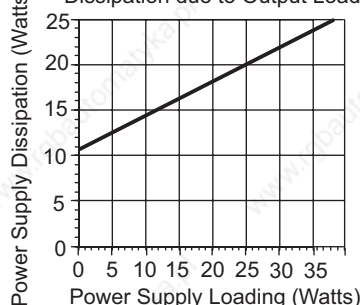
1746-P3 Power Supply Change in Power Dissipation due to Output Loading
