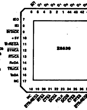
Chip Carrier Pin Assignments, Z8530
