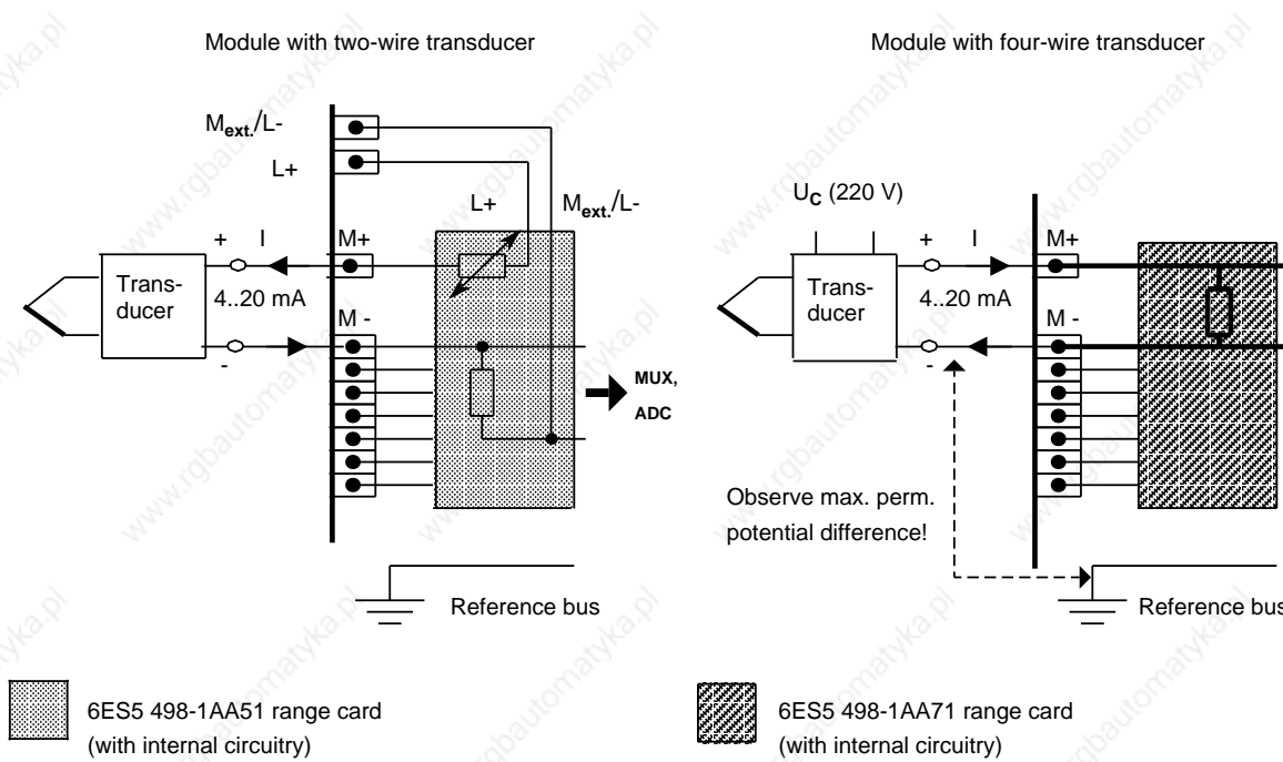
Figure 10-8. Connecting Transducers
