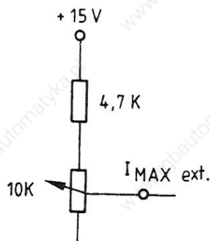
Fig. 3.7/2 Presetting of the external current limitation voltage
