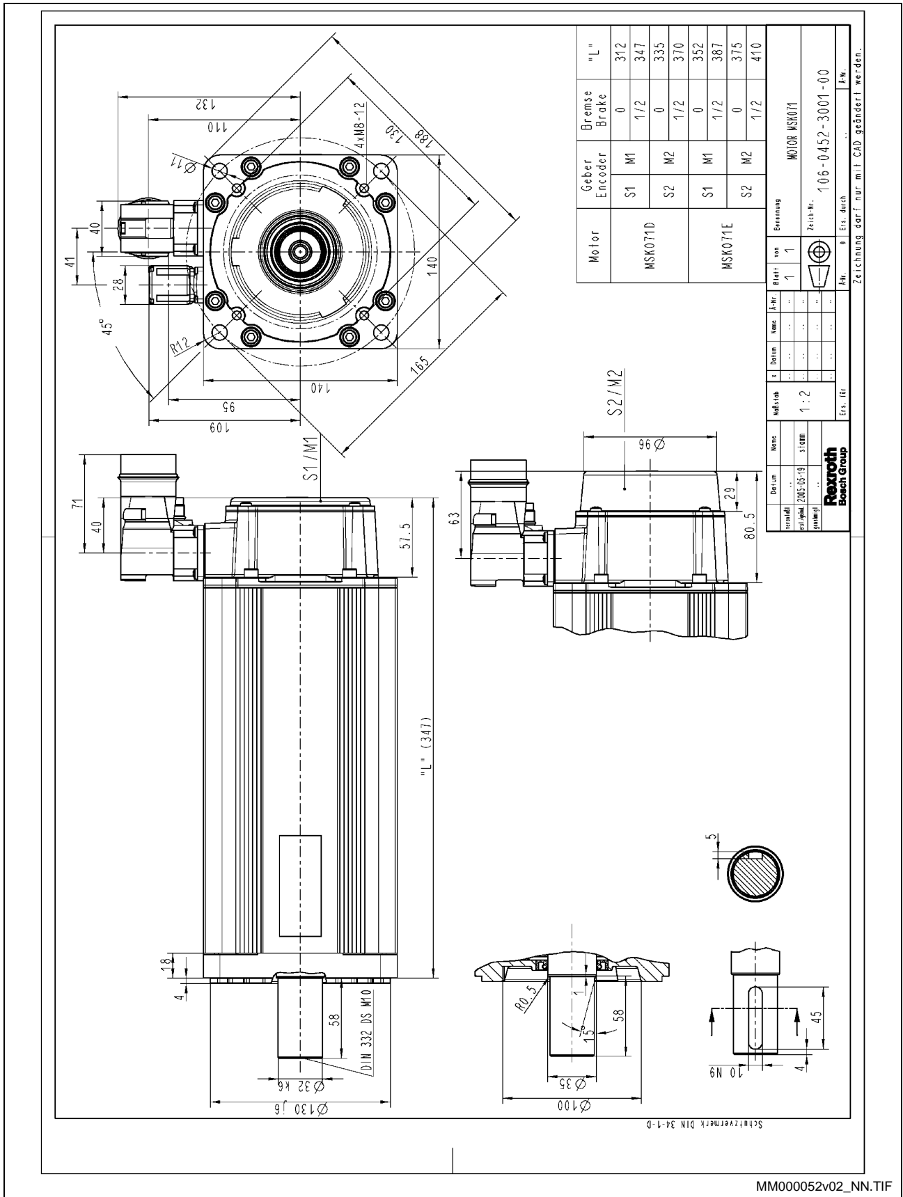
Fig. 5-7: MSK071...NN specification
