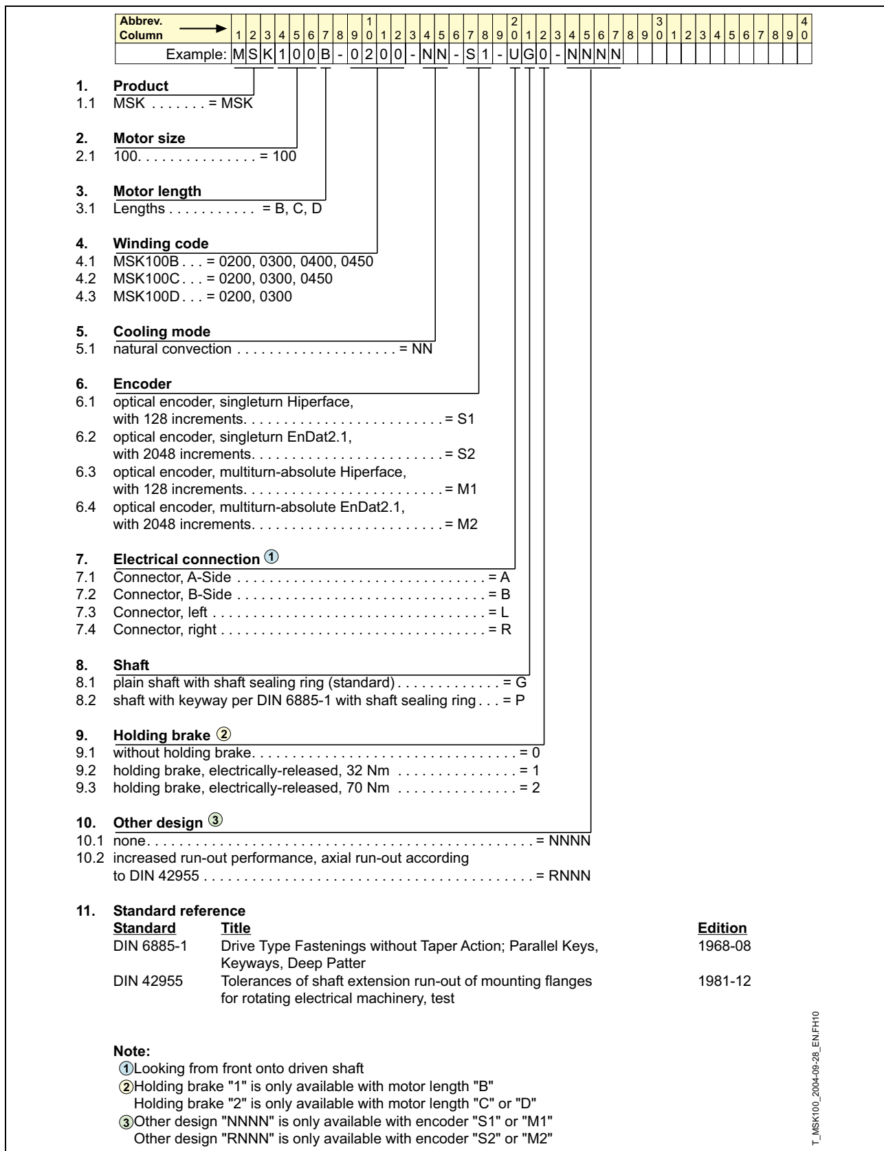
Fig. 6-13: Type code MSK100
