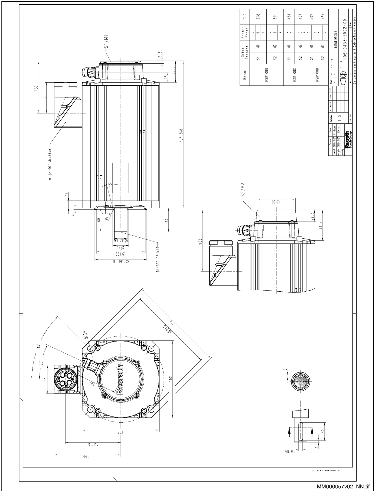
Fig. 5-9: MSK100 specification
