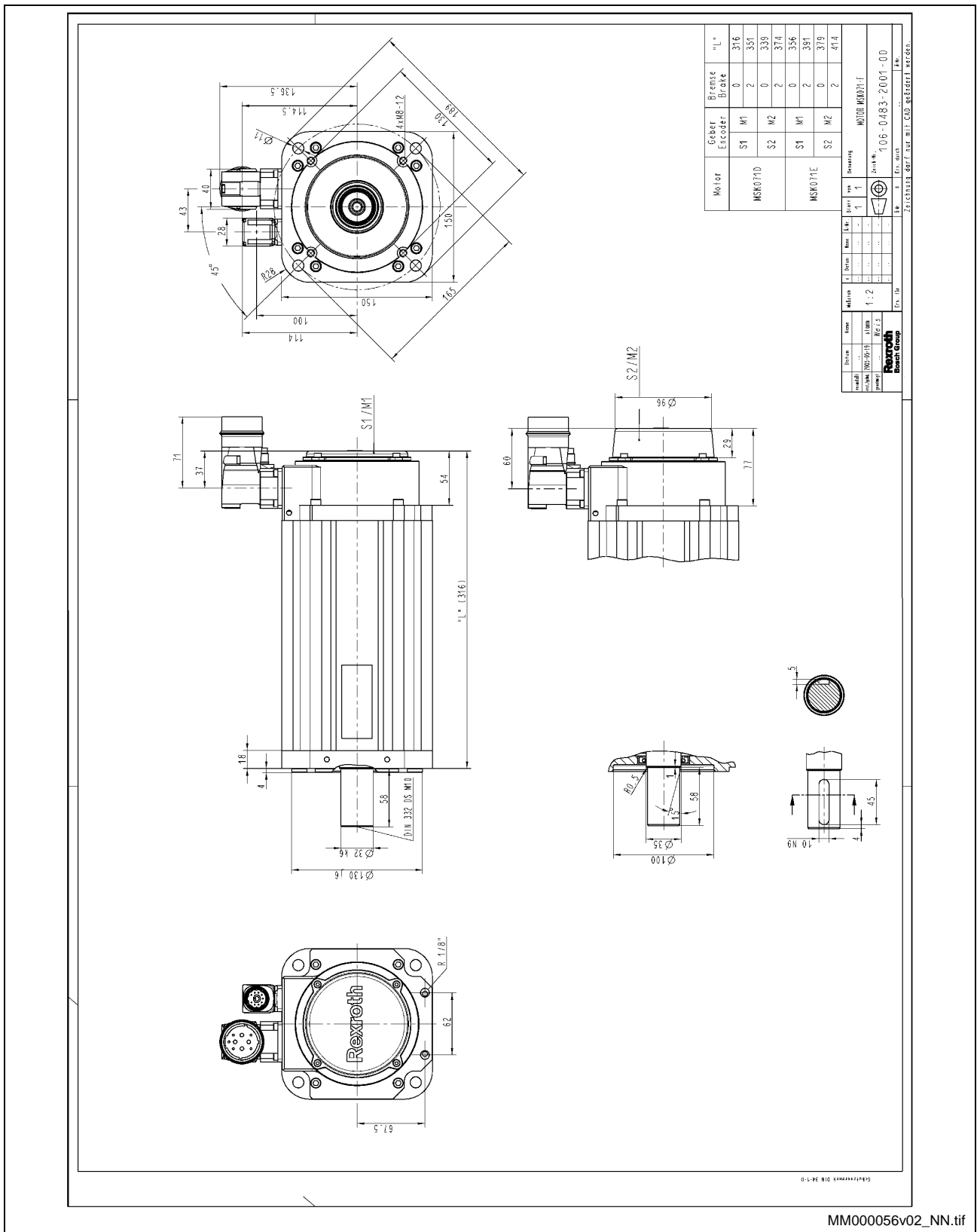
Fig. 5-8: MSK071...FN specification
