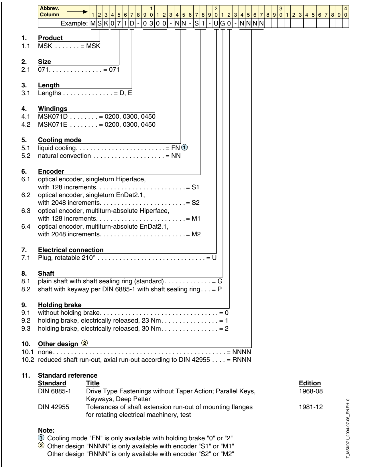
Fig. 6-12: Type code MSK071
