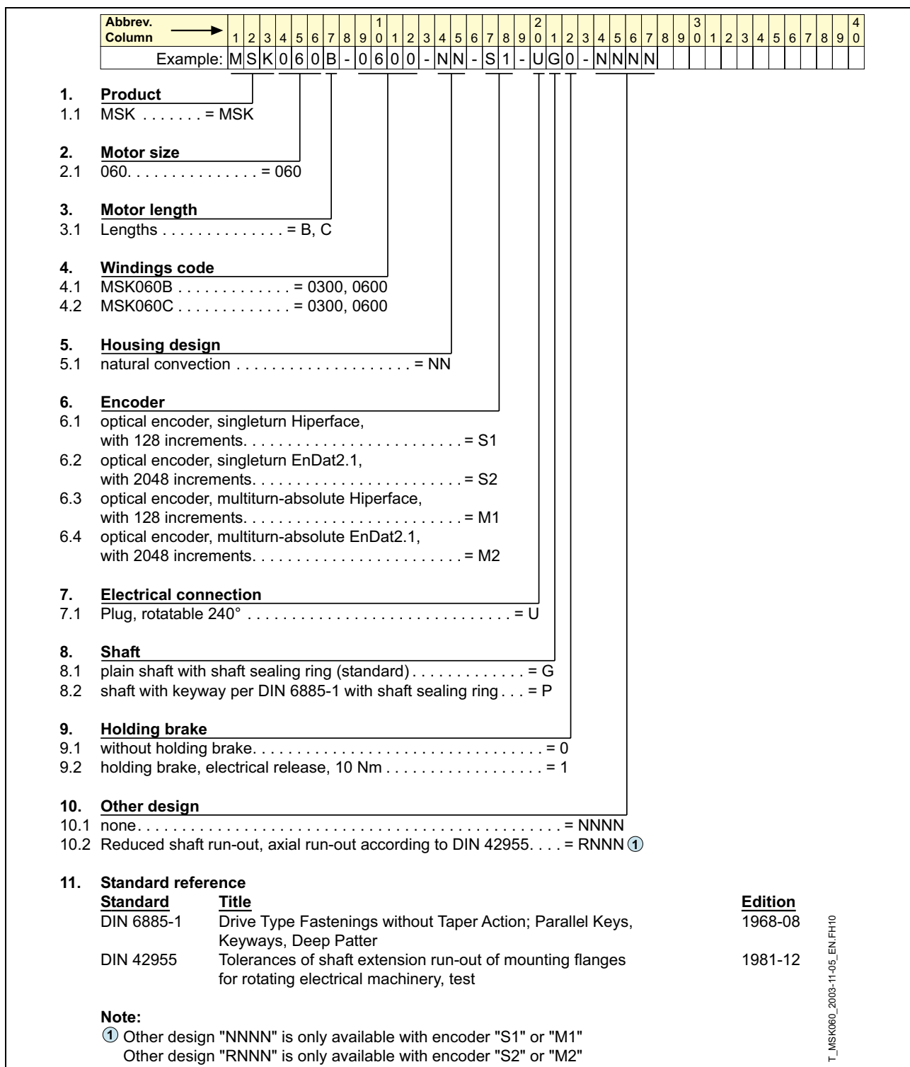
Fig. 6-10: Type code MSK060
