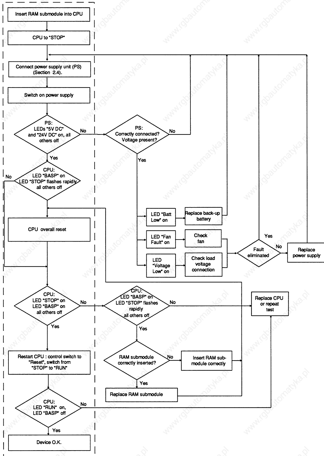
Fig. 15 Starting up
