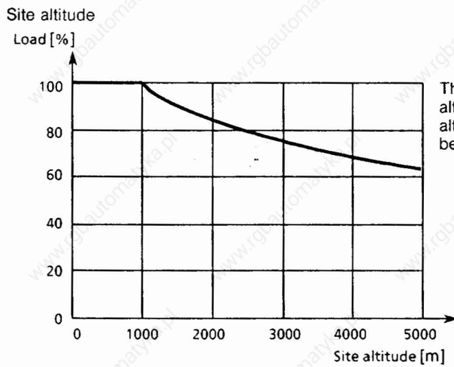
Fig. 1.5 Derating at site altitudes > 1000 m above sea level
