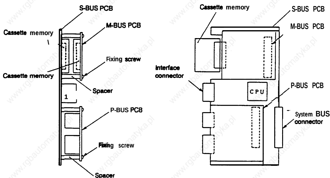
Fig. 1.22 Example of control module (integrated PCB)
