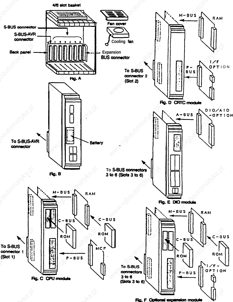
Fig. 1.2.1 Control unit configuration diagram
