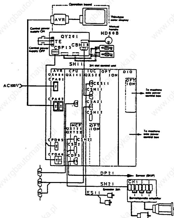
Fig. 4.3 General system drawings (for reference)
