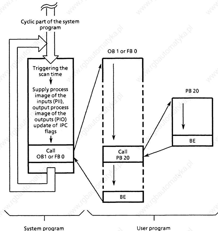
Fig. 14 Cyclic program execution
