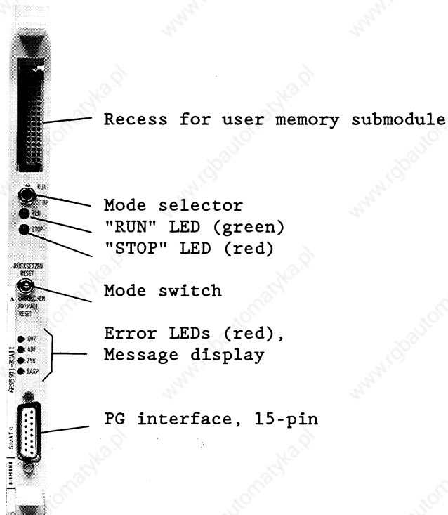
Fig. 2 Front panel of the S processor
