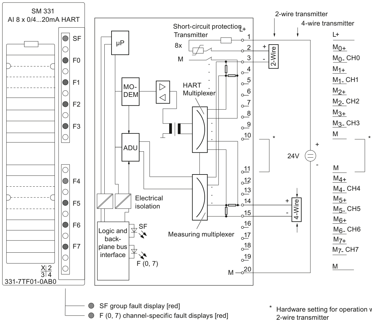
Figure 6-1 Module view and schematic circuit diagram of the SM 331; AI 8 x 0/4...20mA HART
