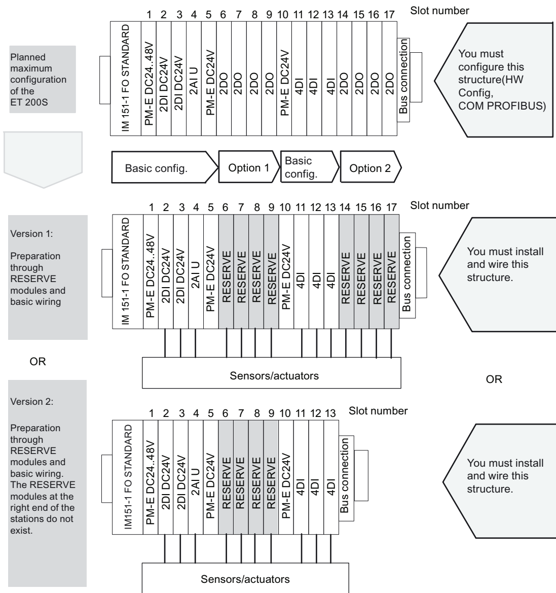
Figure 3-2 Example for using RESERVE modules
