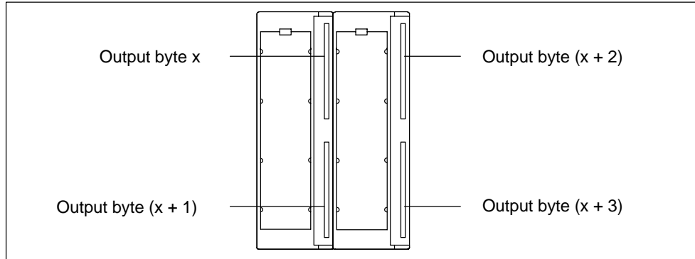
Figure 3-17 Terminal Assignment of the SM 322; DO 32 × 120 VAC/1.0 A
