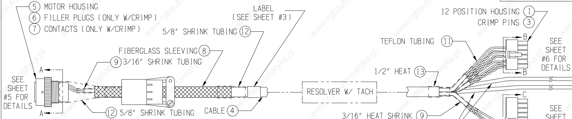
TUBING & SLEEVING PARTS LIST (FOR CONNECTORS & RELATED PARTS, SEE INDIVIDUAL SHEETS)
