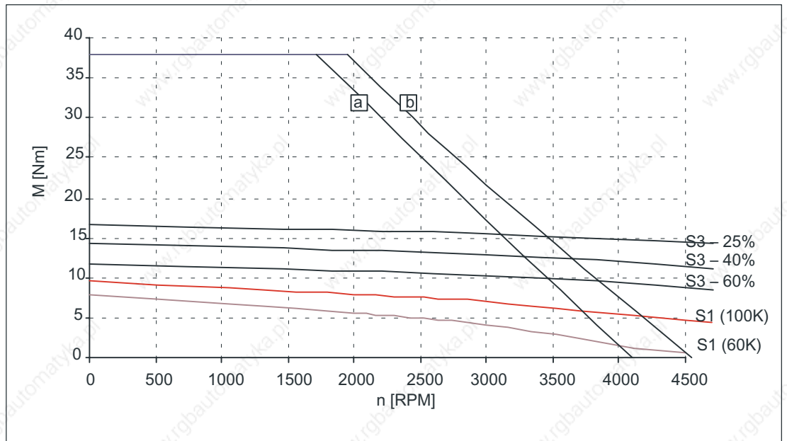
Figure 3-18 Speed-torque diagram 1FT6064-6AF7
