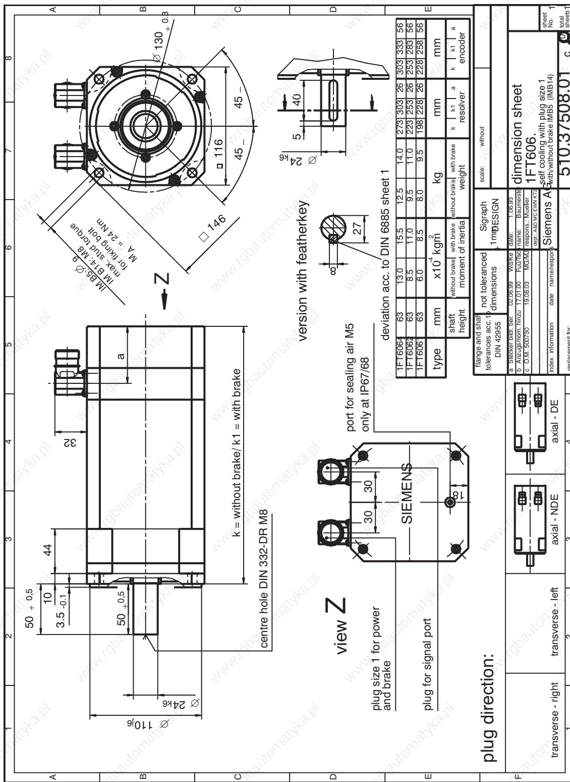
Figure 5-20 1FT6064 non-ventilated with connector, Size 1
