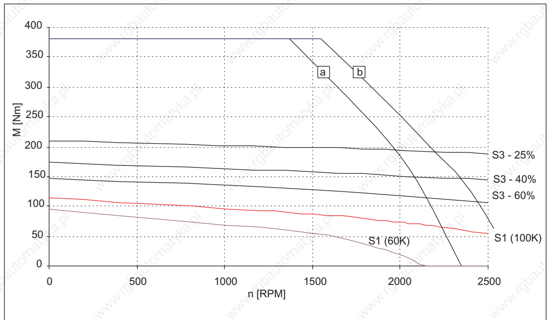
Figure 3-52 Speed-torque diagram 1FT6136-6AC7
