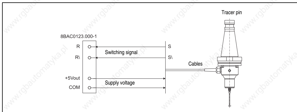
Figure 172: Connection example for cabled tracer pins with 5V supply and TTL output signals
