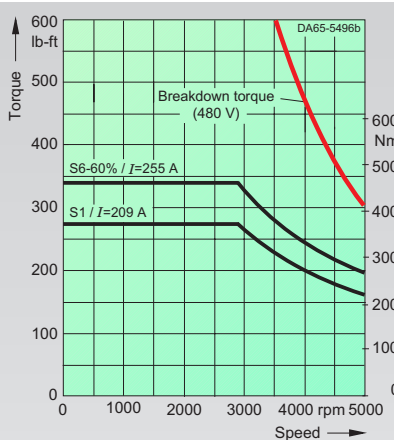
1PL6184-4.L. max. breakdown torque: 904 lb-ft/1226 Nm
