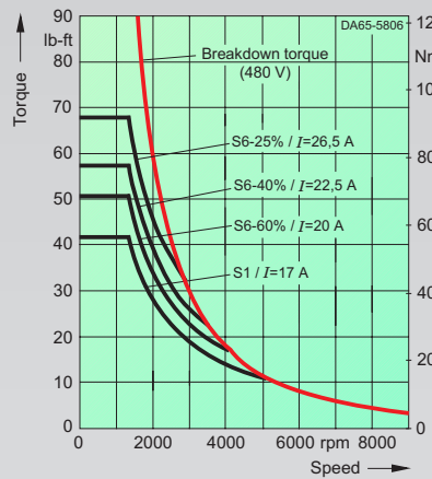
1PH7107-2.D...-.... max. breakdown torque: 100 lb-ft/135 Nm
