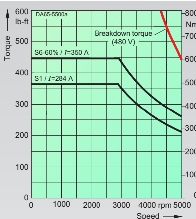
1PL6186-4.L. max. breakdown torque: 1330 lb-ft/1803 Nm
