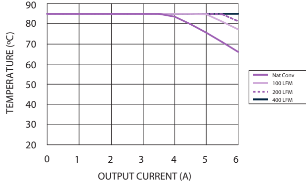
Figure 1 - Safe Operating Area for PTH12050W V_{in} = 12\text{ V} , Output Voltage = 3.3 V (See Note A)
