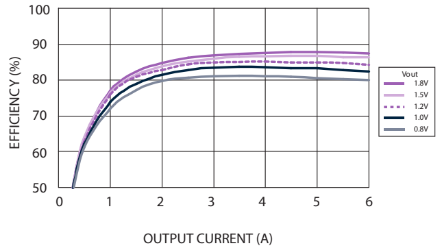
Figure 4 - Efficiency vs Load Current for PTH12050L V_{in} = 12\text{ V} (See Note B)
