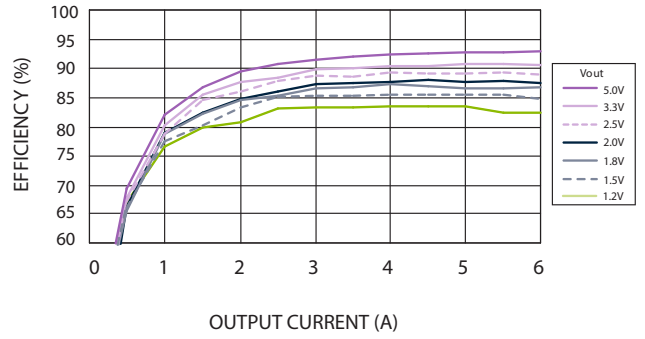
Figure 2 - Efficiency vs Load Current for PTH12050W V_{in} = 12\text{ V} (See Note B)
