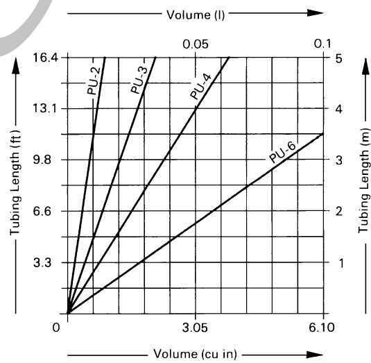
Evacuation volume as a function of the number of suction cups (VAS) and tubing (PU)
