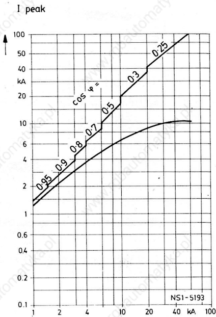
Short circuit current I_k (effective)
